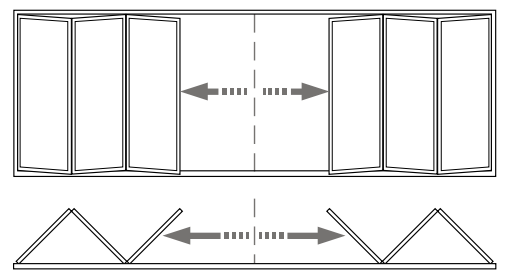
Visofold doors fold to give large opening aperture.
