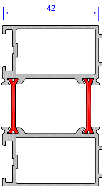
DV32 Meeting stile for non-swinging doors
