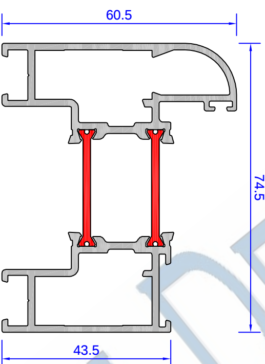
DV26 Door sash (Open In & Out)
