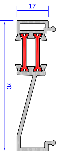
DV172 17mm Add-On / Drainage Tray
