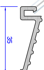
EUD03 Ramp for DV171 low threshold (Only available in silver anodised finish.)
