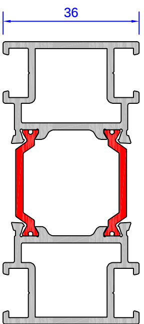
DV32 Meeting stile for non-swinging doors
