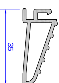
DV174: Ramp for DV173 low threshold (Only available in silver anodised finish.)
