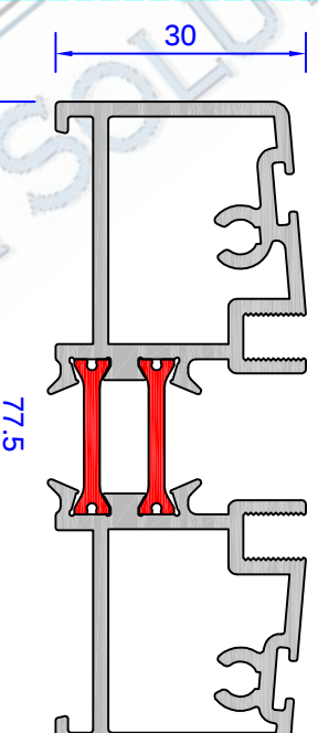
*DV175 Flush Threshold
