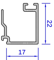
DV67 28mm Glazing Bead
