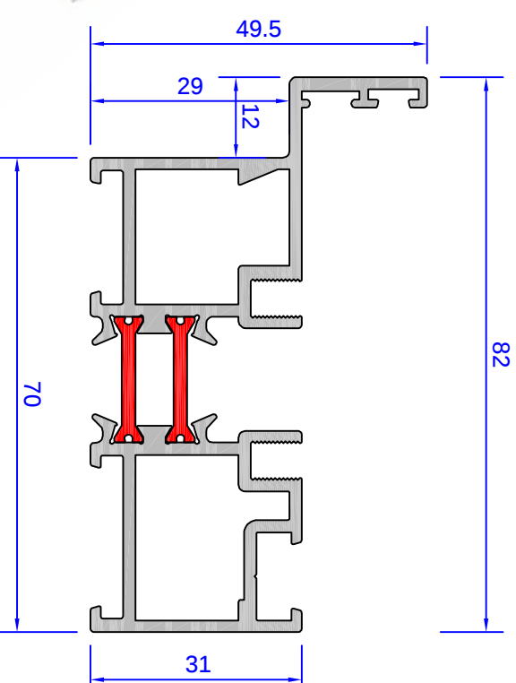
DV14N Outer Frame (Open In & Out)
