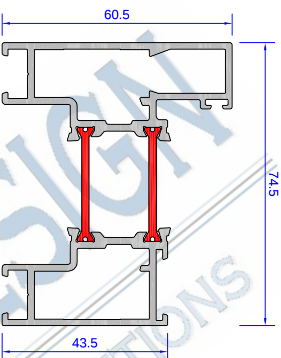
DV23 Door sash (Open In & Out)
