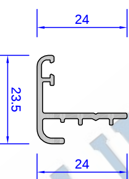
DV56 Rebate for swinging door sash
