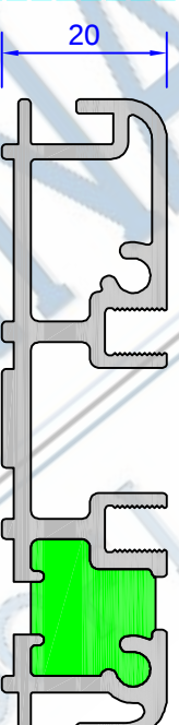
*DV171 Low Threshold (Only available in silver anodised Finish.)
